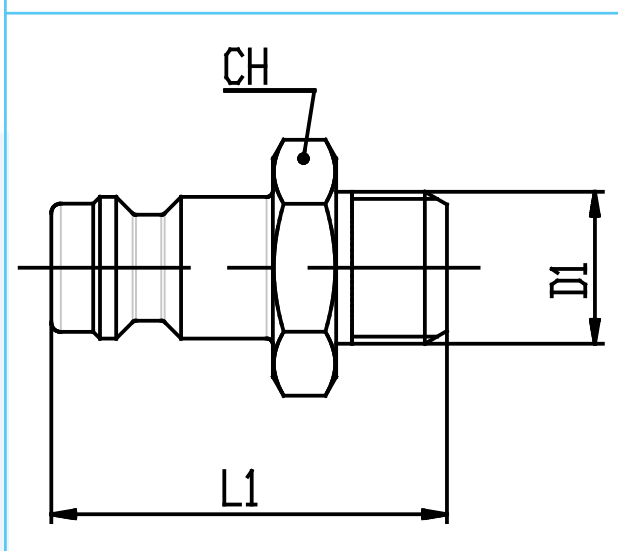
GU21-20 Male Plug
